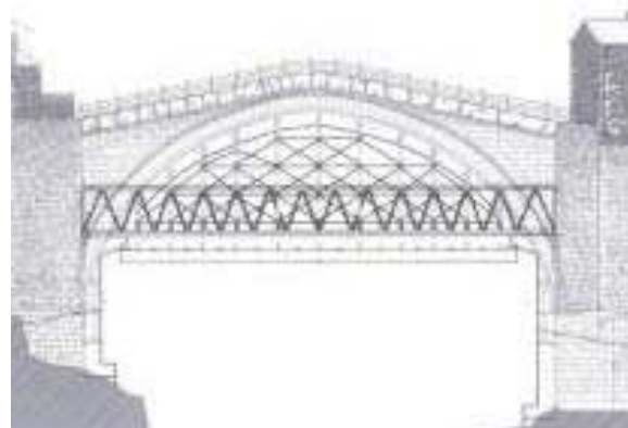
Fig. 9: South elevation of centering
