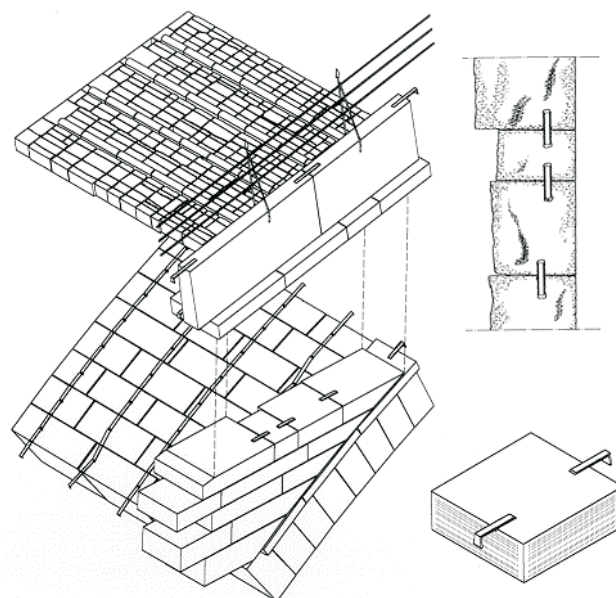
Fig. 17: Scheme of spandrel stone assembly
