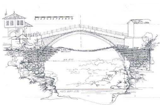
Fig. 25: Presumed appearance of the suspension bridge, by Prof. Gojkovic
