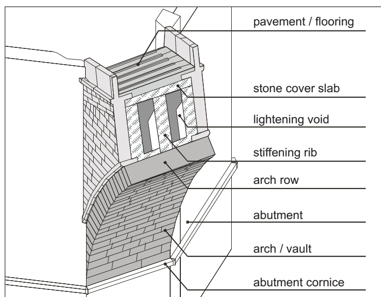
Fig. 6: Structural elements of the bridge
