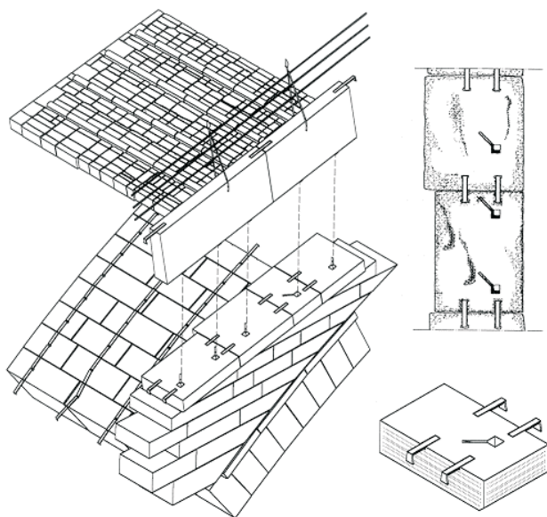
Fig. 19: Scheme of the upper cornice assembly
